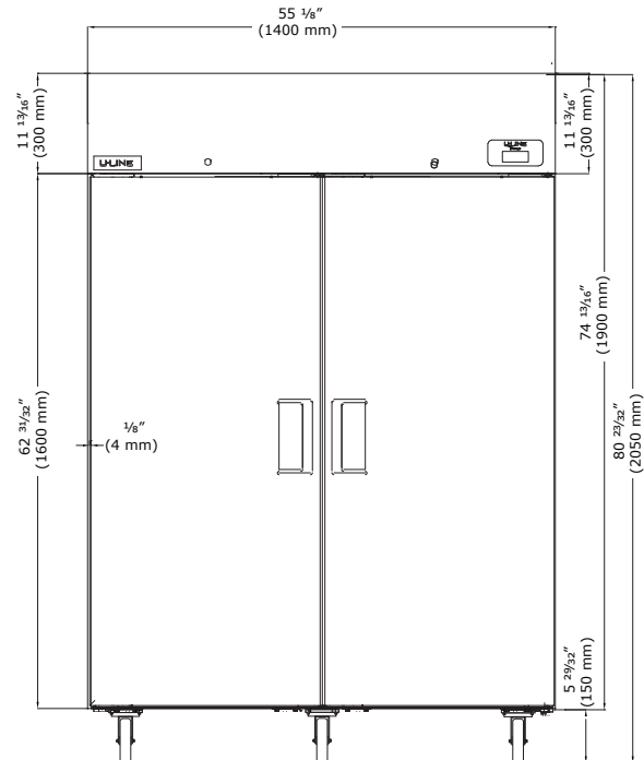
Front (Closed)
